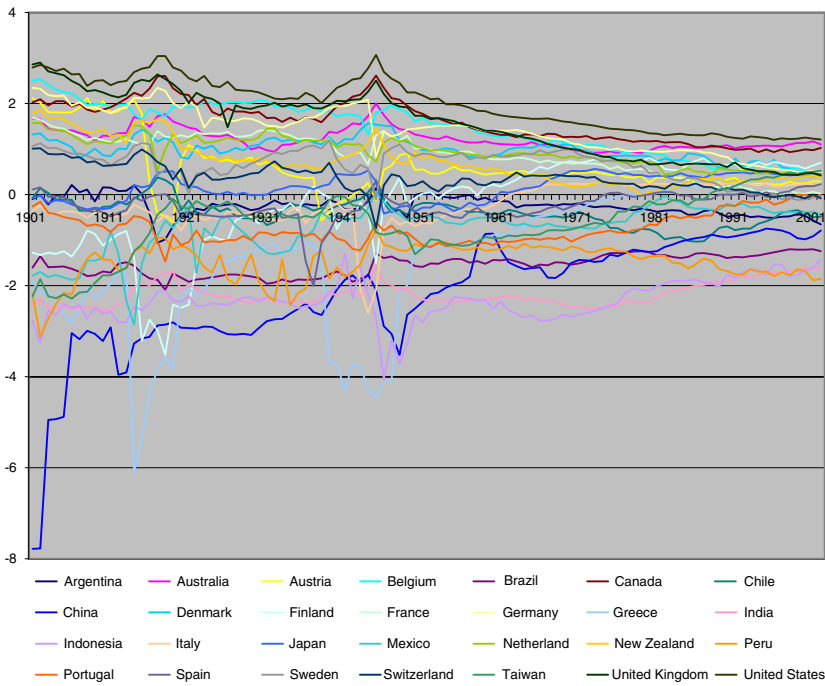
Fig. 1 Cross-sectionally demeaned CO 2 emissions for the G28 panel
